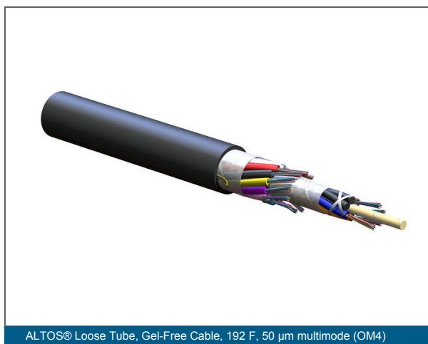
ALTOS® Loose Tube, Gel-Free Cable, 192 F, 50 µm multimode (OM4)
