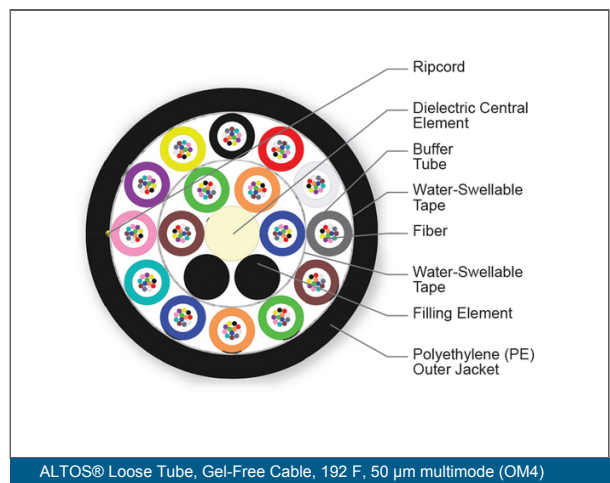
ALTOS® Loose Tube, Gel-Free Cable, 192 F, 50 µm multimode (OM4)
